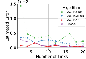
Fig. 10. Bit-Flip - Estimation Error vs Path Number
