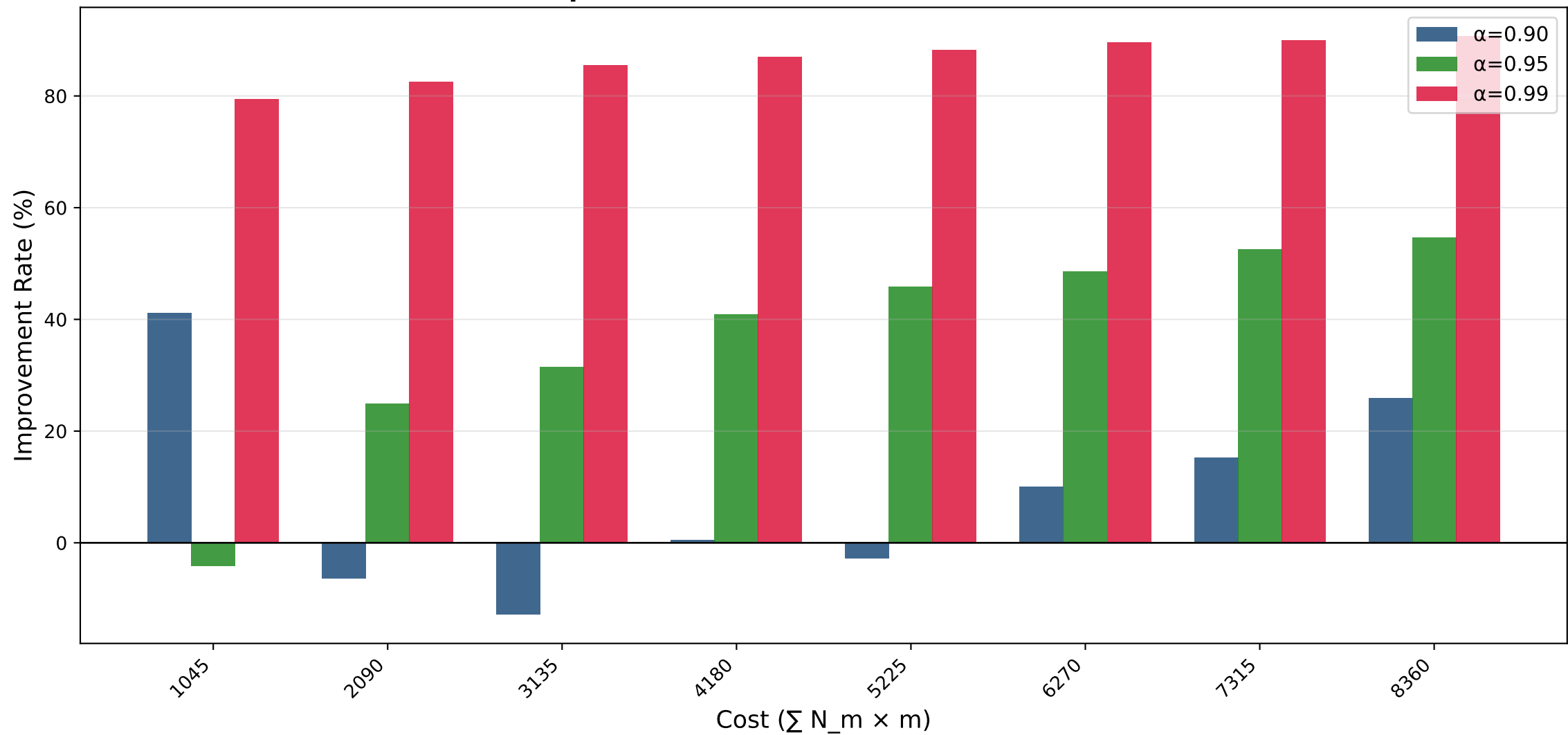
WLS Improvement Rate vs Cost - Bar Plot (m2-20)
