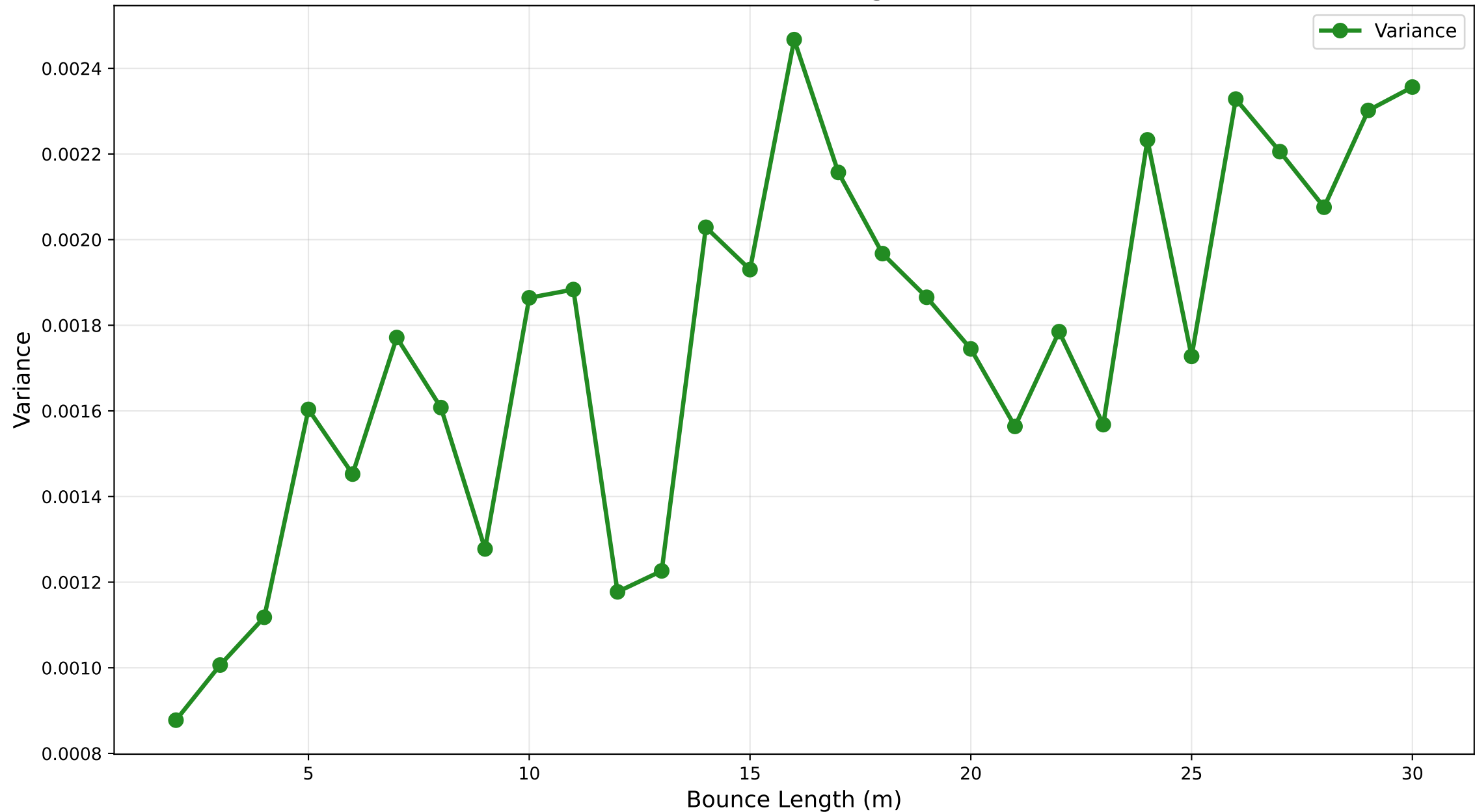
Variance vs Bounce Length ( \alpha=0.95 )
