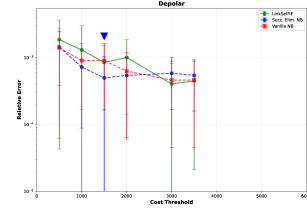
Fig. 6. Depolarizing - Significance Visualization
