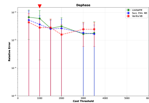
Fig. 5. Dephasing - Significance Visualization
