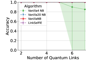
Fig. 11. Amplitude Damping - Accuracy vs Path Number
