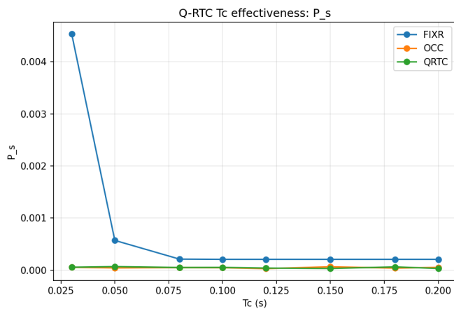
Fig. 4. Stall probability under different coherence deadlines.
