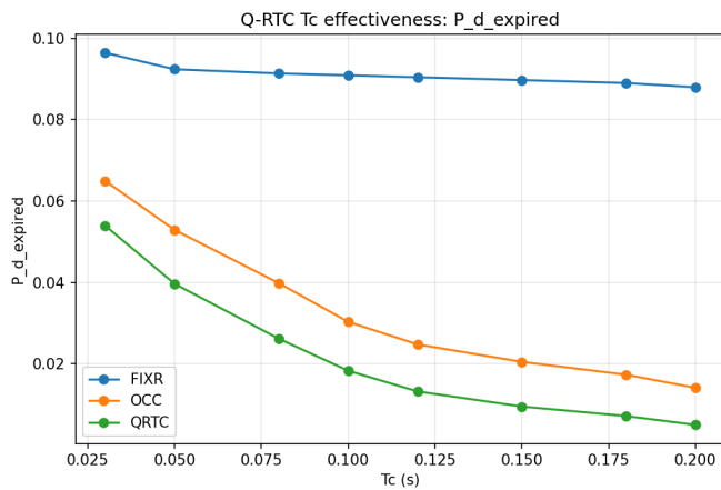
Fig. 3. Discard probability under different coherence deadlines.
