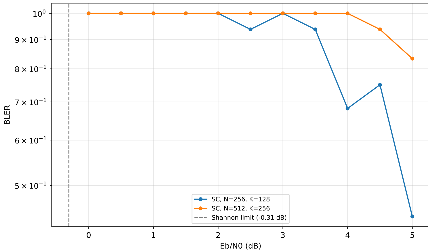
SC BLER
