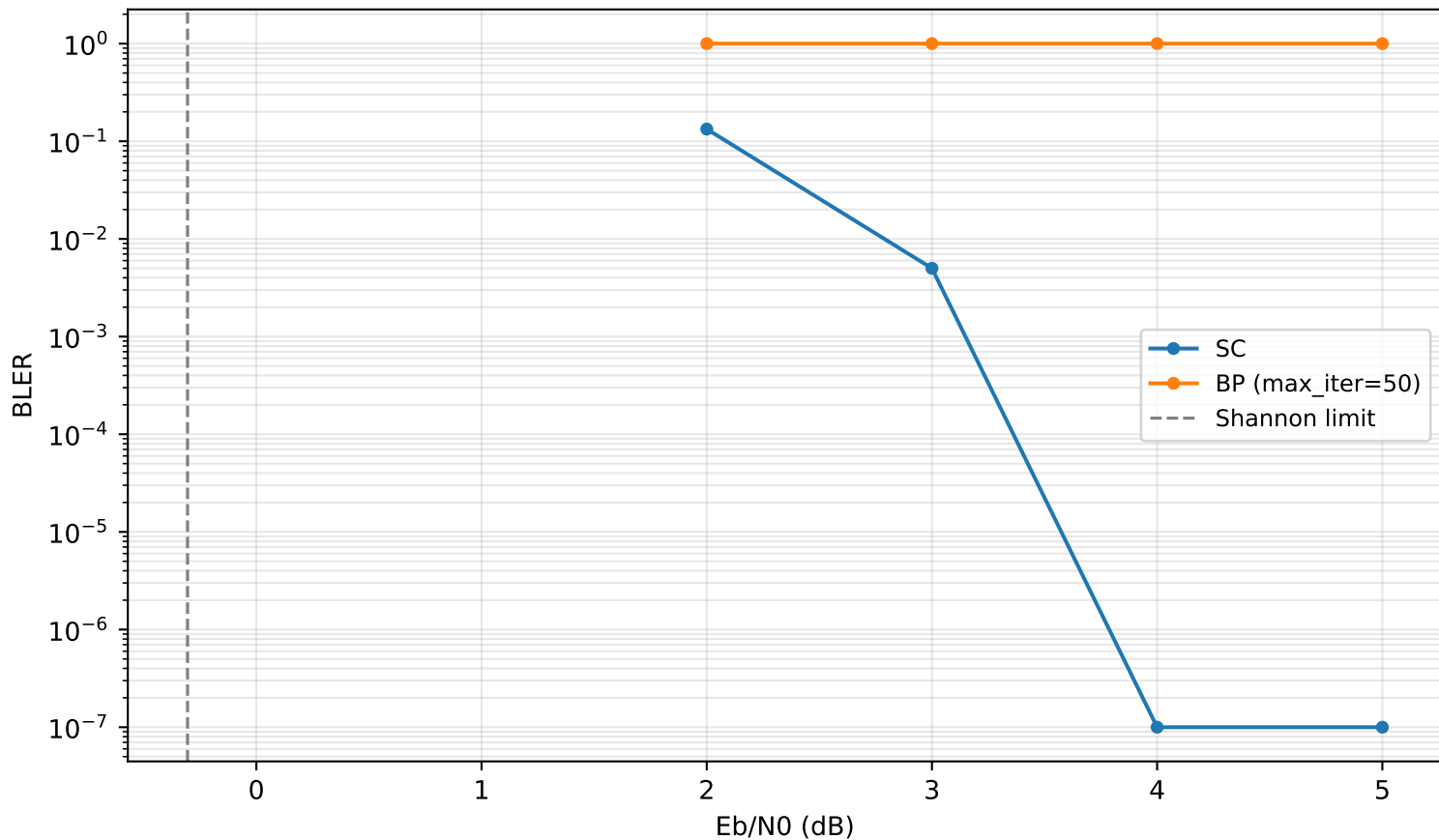
SC vs BP (N=512, R=0.5)
