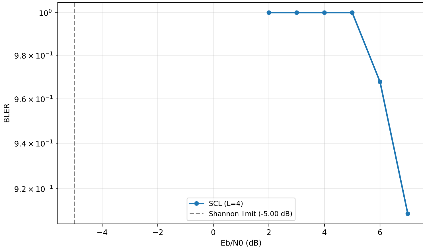
SCL BLER N=512
