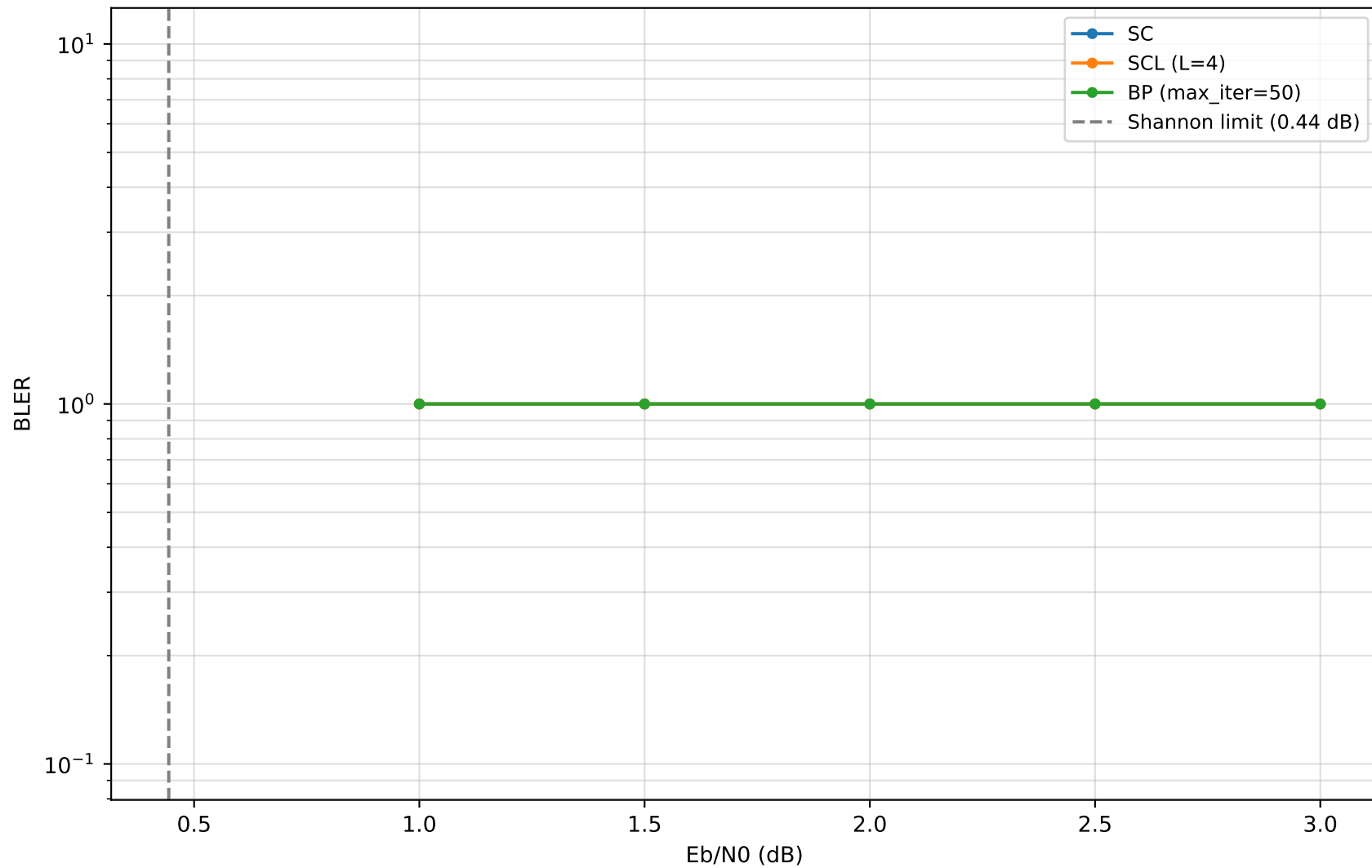
SC vs SCL vs BP (N=128, R=0.5)
