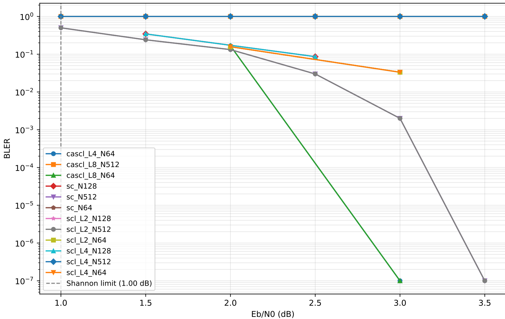
SCL vs SC BLER (R=0.5)
