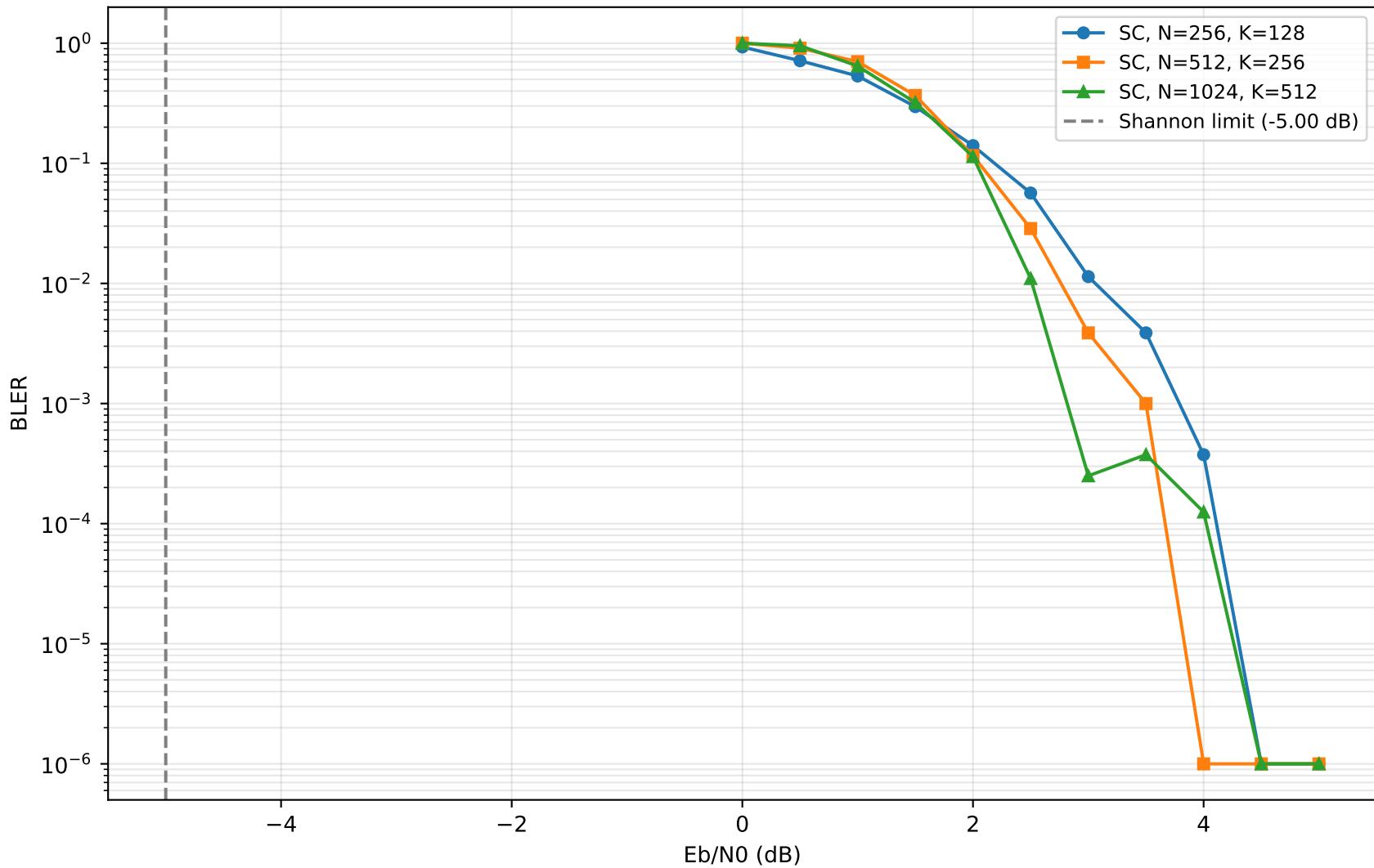
SC BLER (R=0.5)
