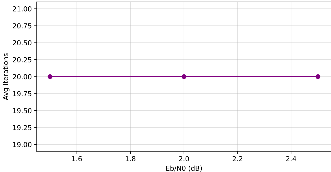
BP Average Iterations (N=64, max_iter=20)
