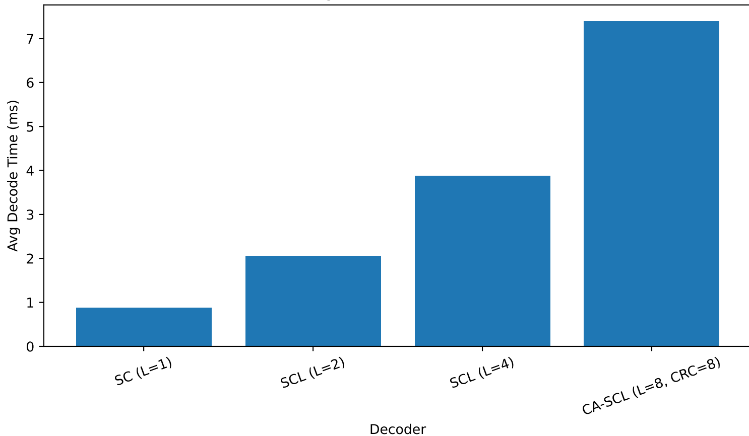
Decoding Time vs List Size (N=64)
