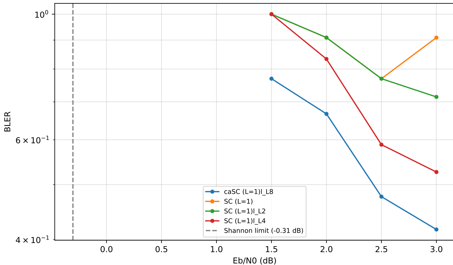
SCL vs SC BLER
