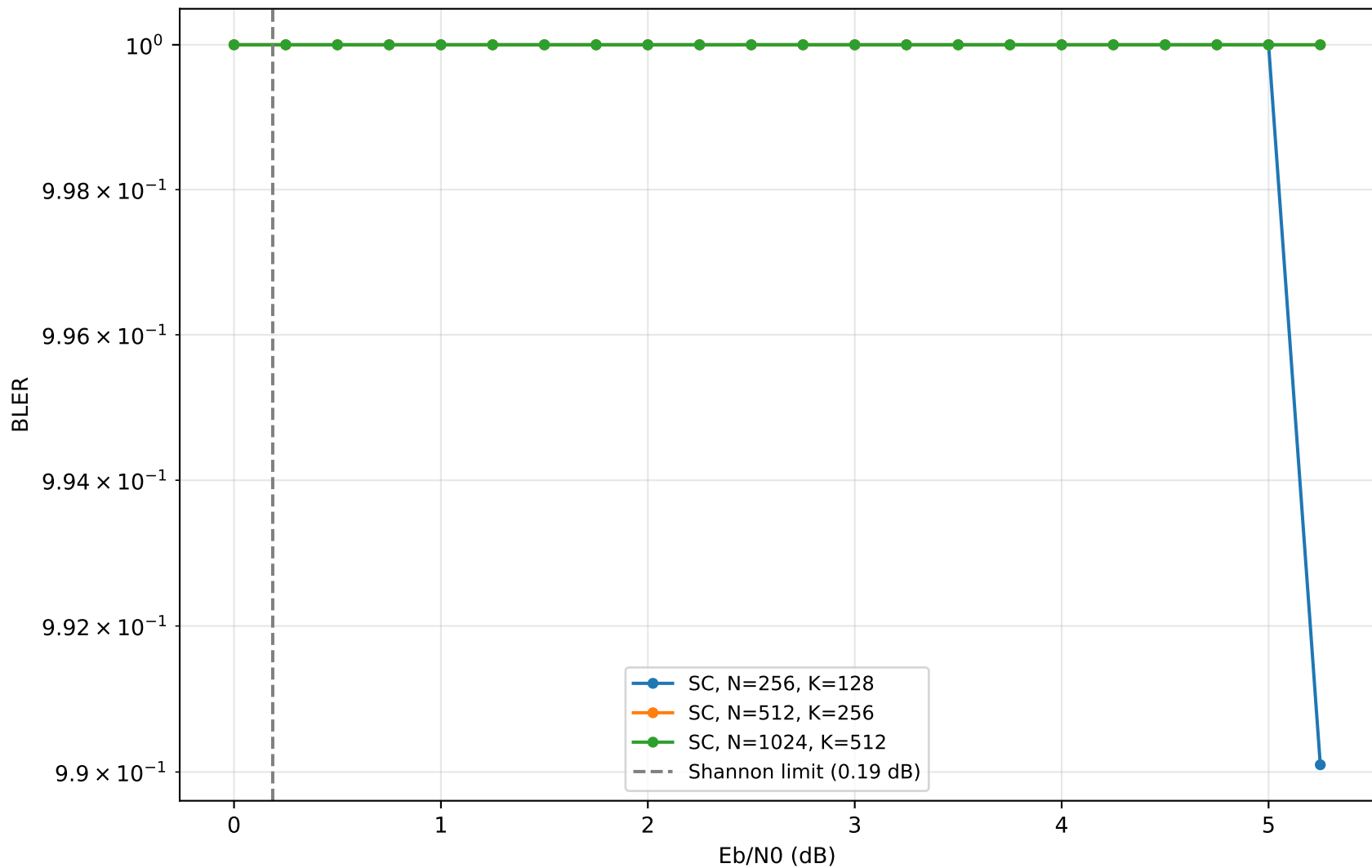
SC Decoder BLER vs Eb/N0 (R=0.5)
