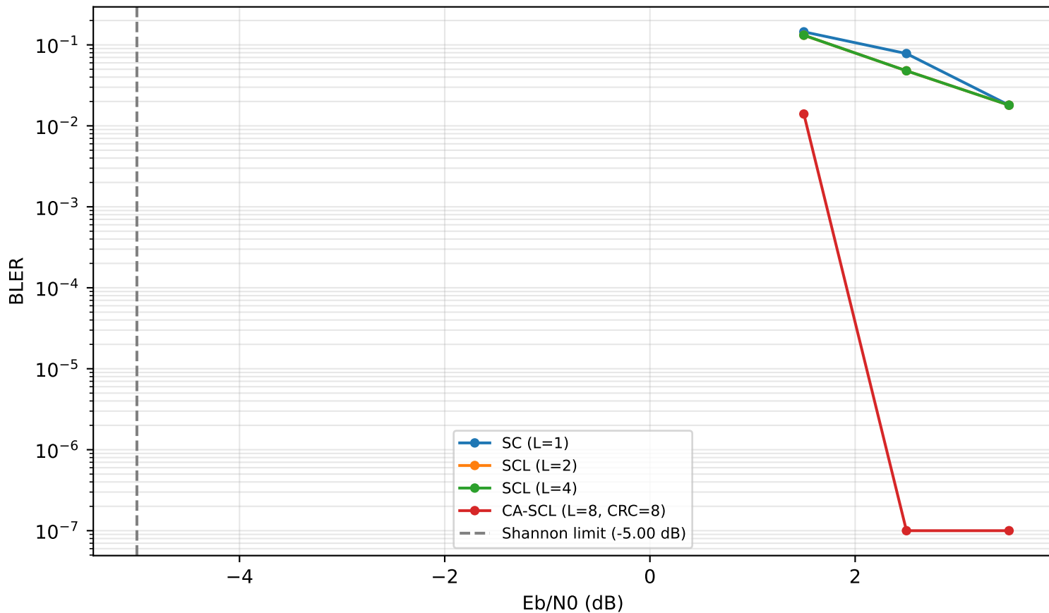
SCL vs SC BLER (N=32, R=0.5)
