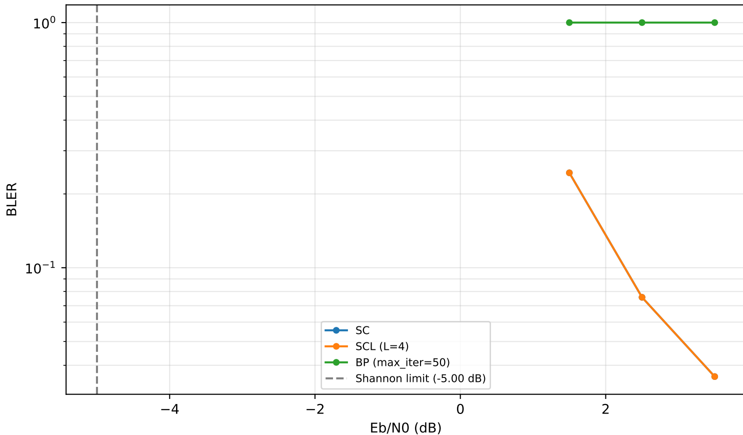
SC vs SCL vs BP (N=16, R=0.5)
