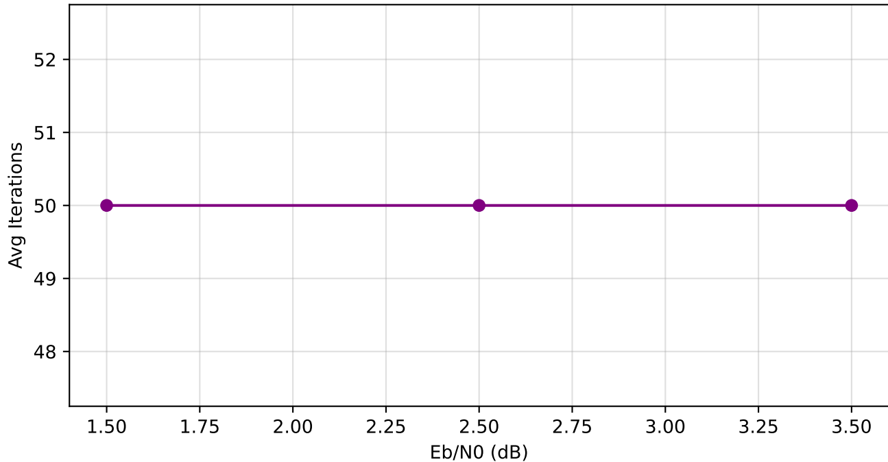
BP Average Iterations (N=16, max_iter=50)
