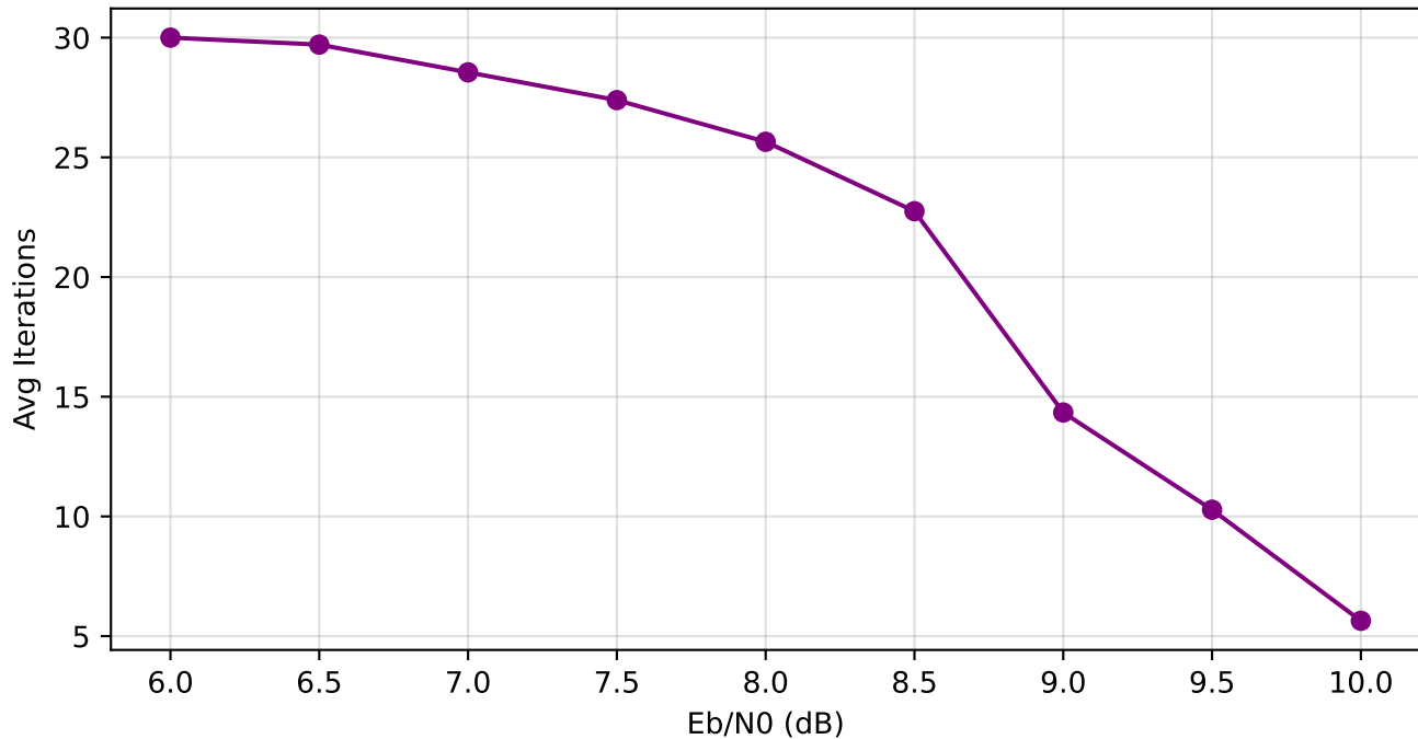
BP Average Iterations (N=256, max_iter=30)
