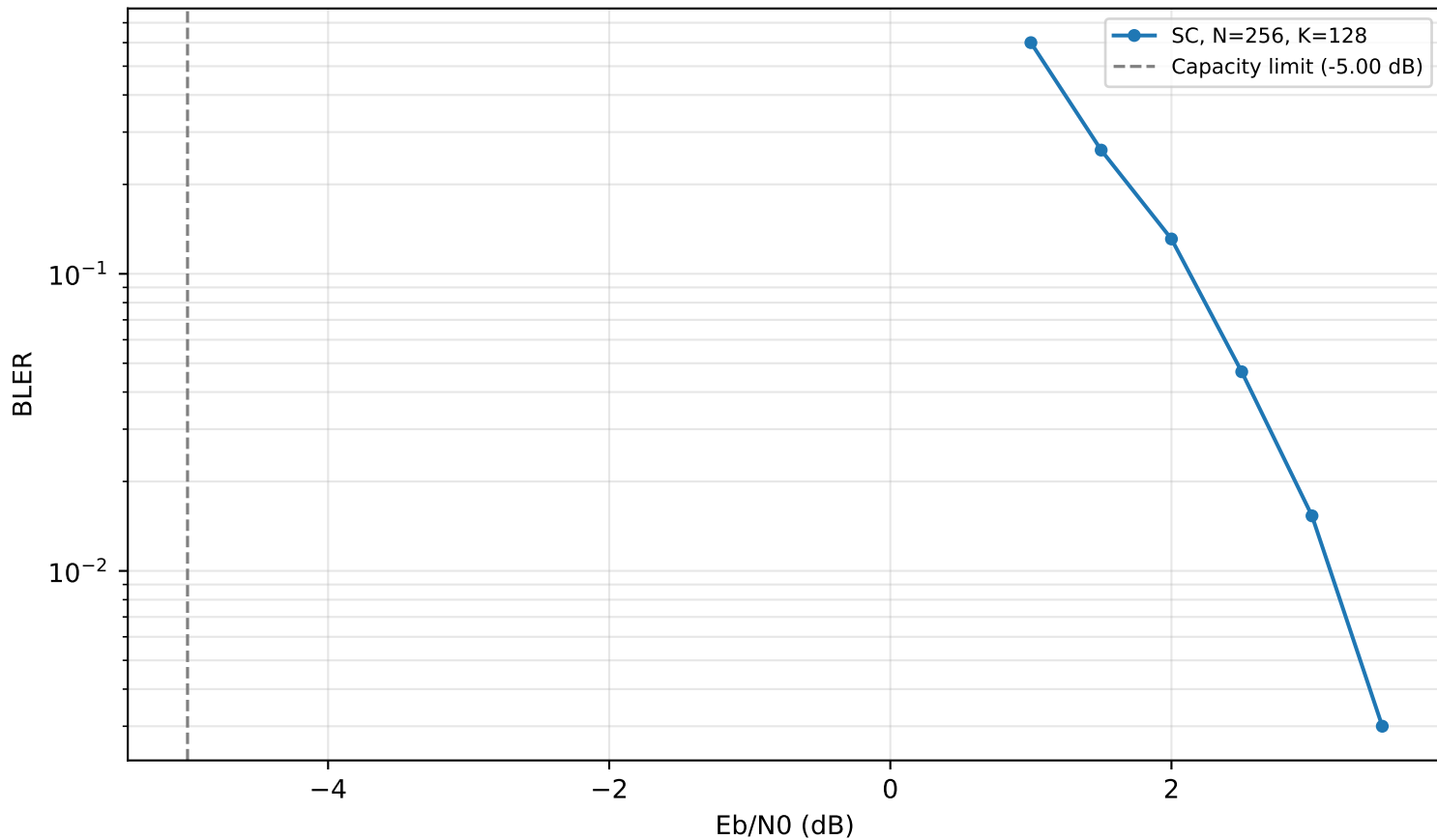
SC Decoder BLER (smoke test)
