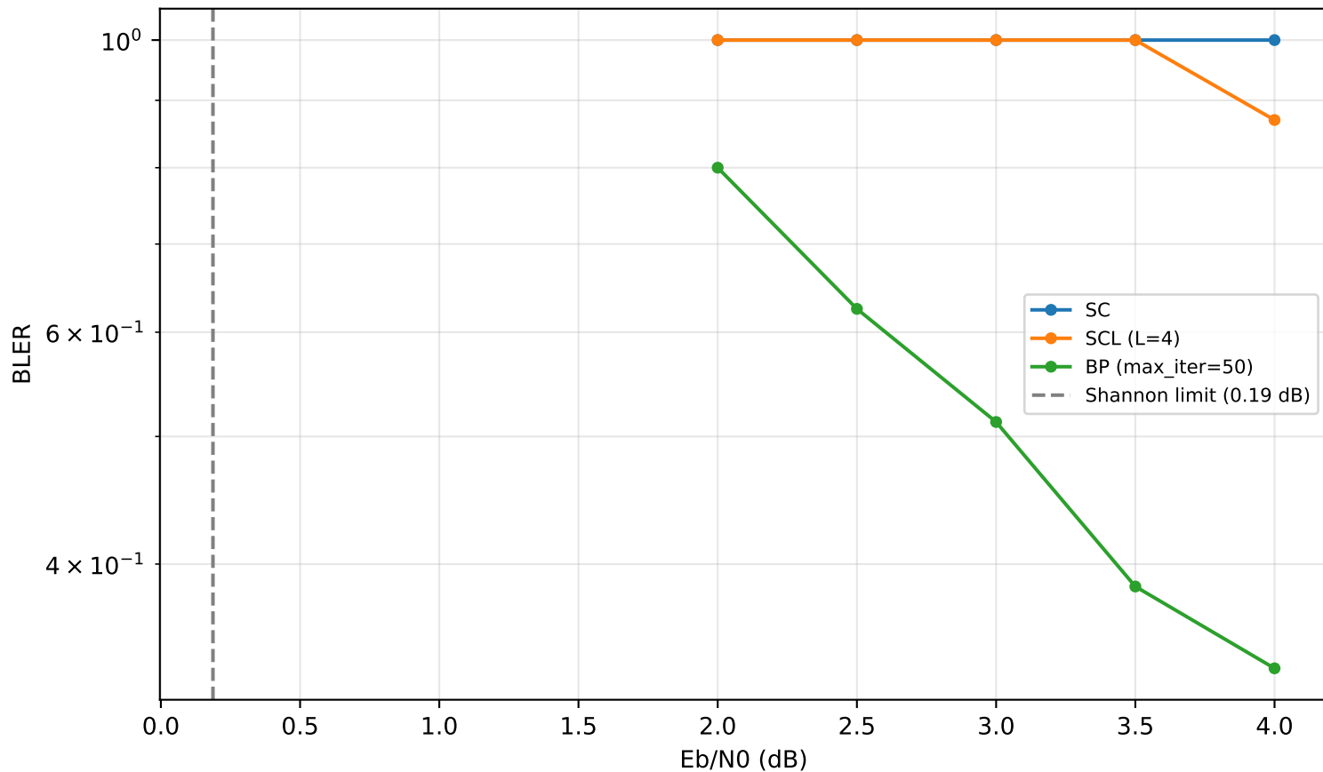
SC vs SCL vs BP (N=128, R=0.5)
