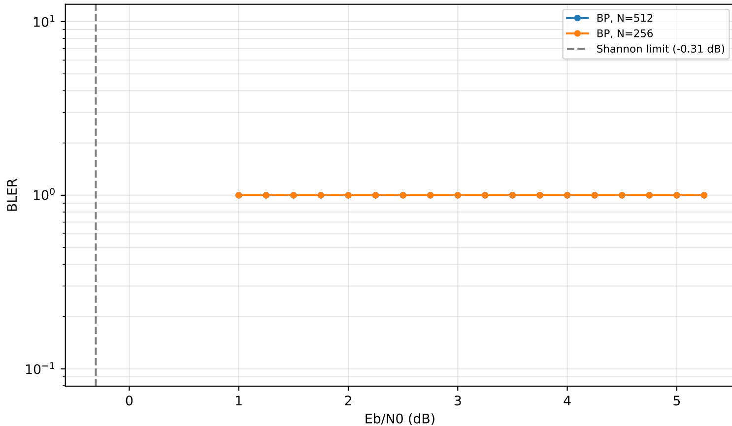
BP Decoder BLER
