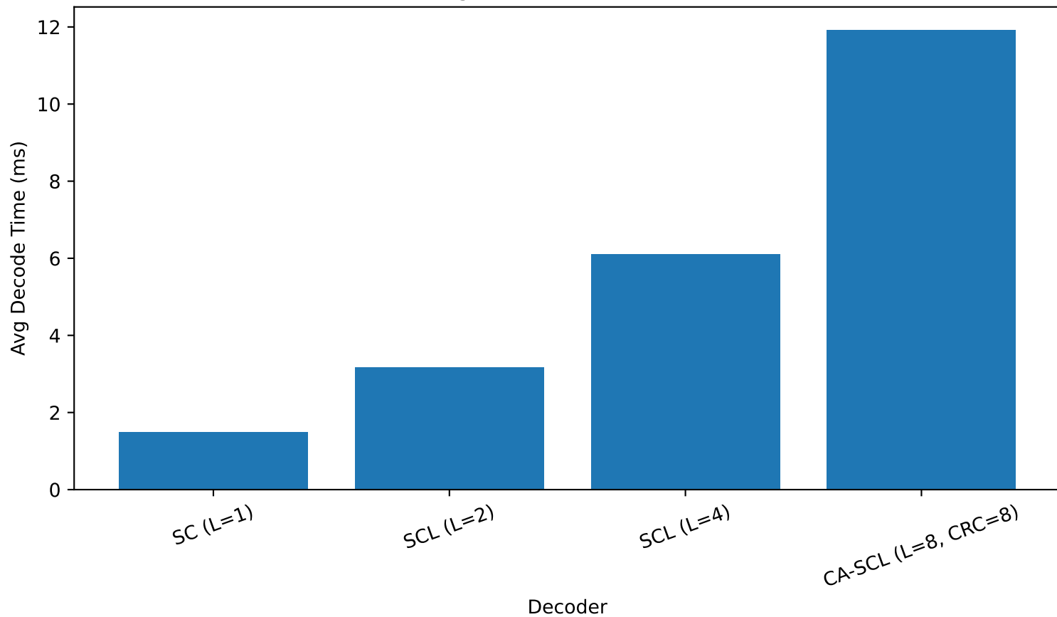
Decoding Time vs List Size (N=128)
