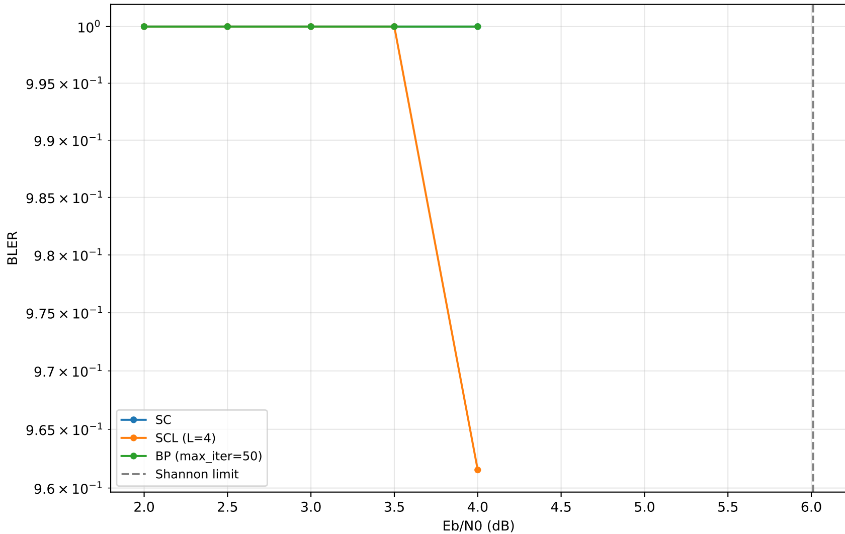
SC vs SCL vs BP (N=256, R=0.5)
