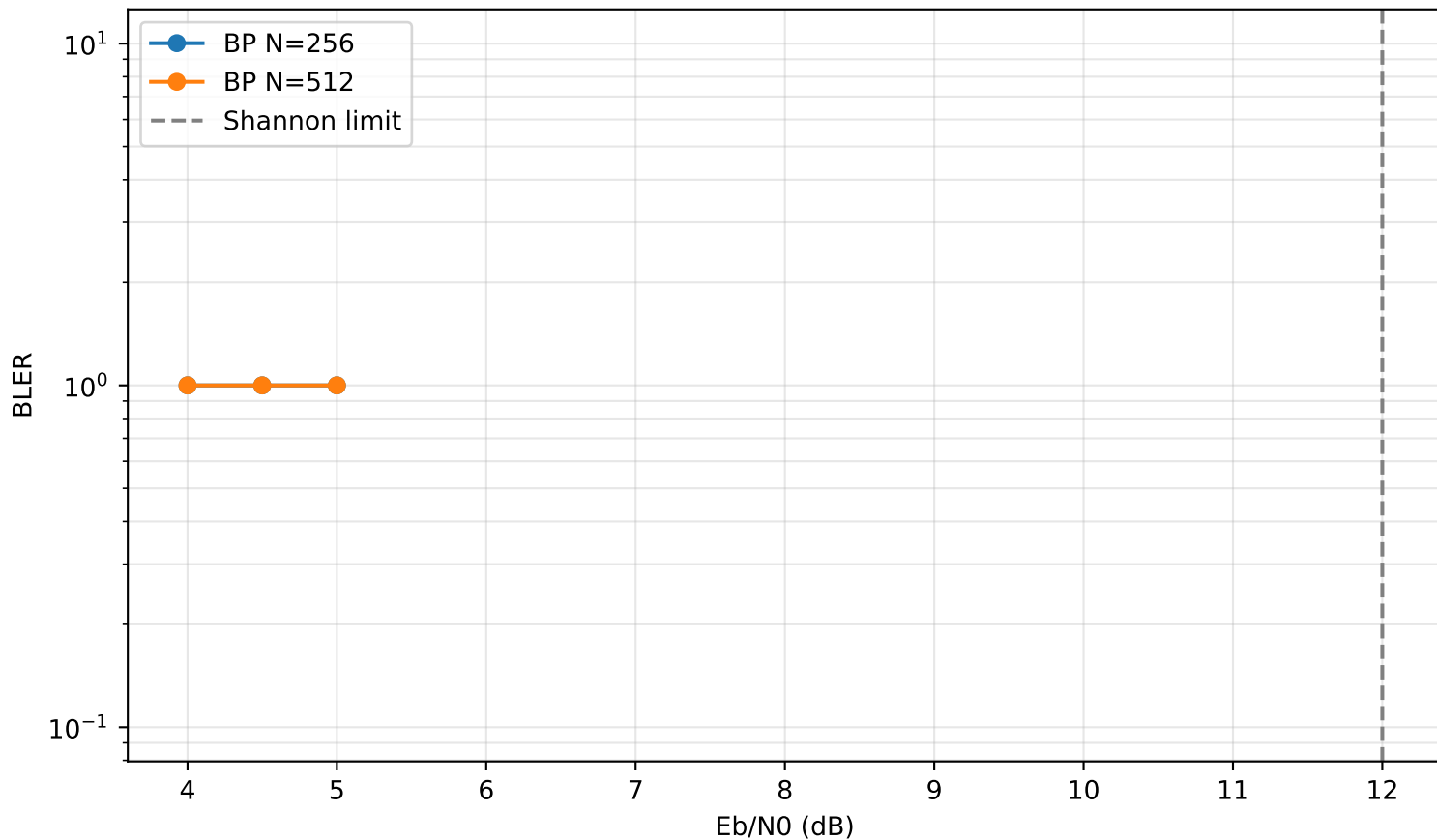
BP Decoder BLER (R=0.5)
