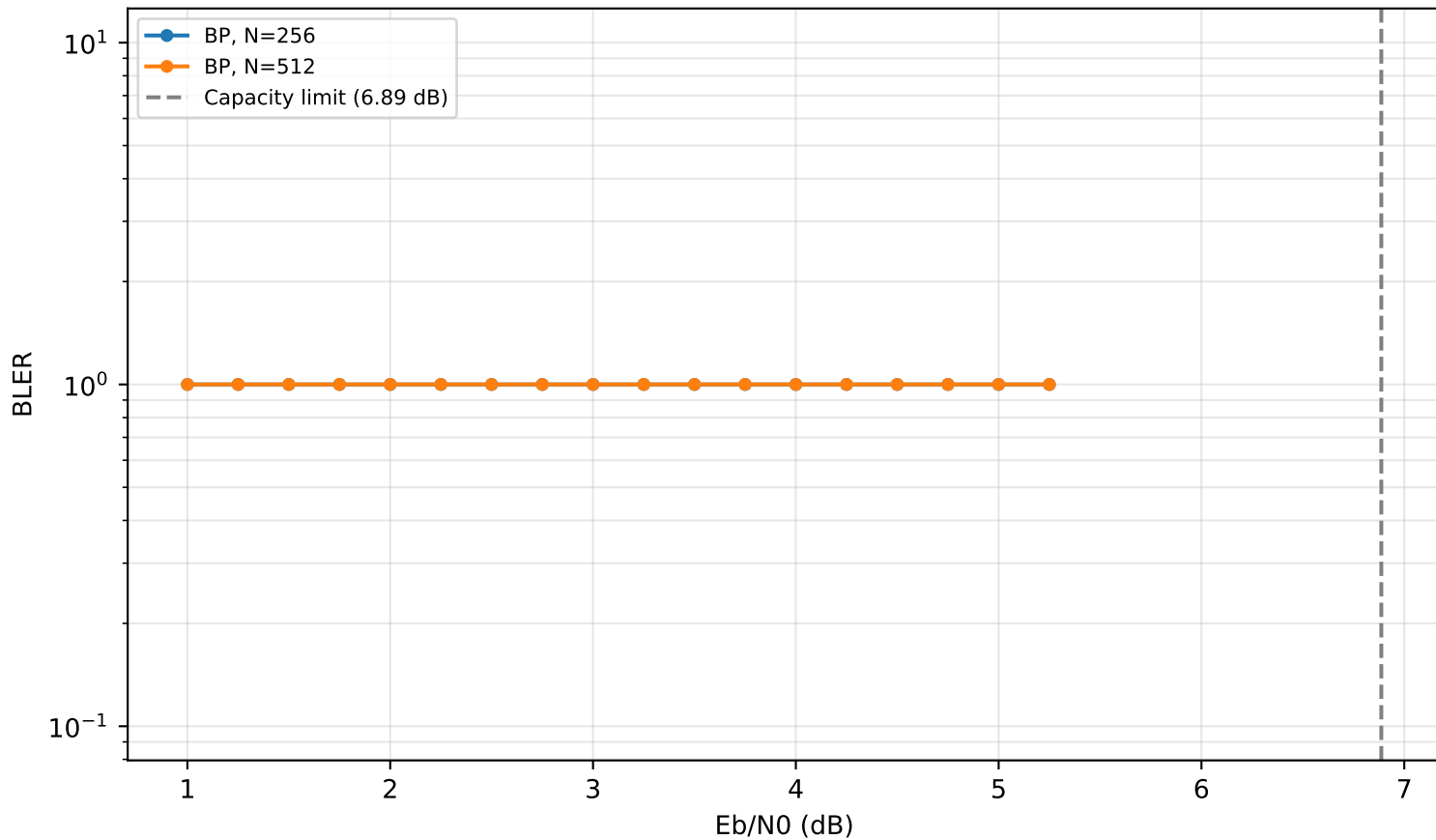
BP Decoder BLER vs Eb/N0 (R=0.5)
