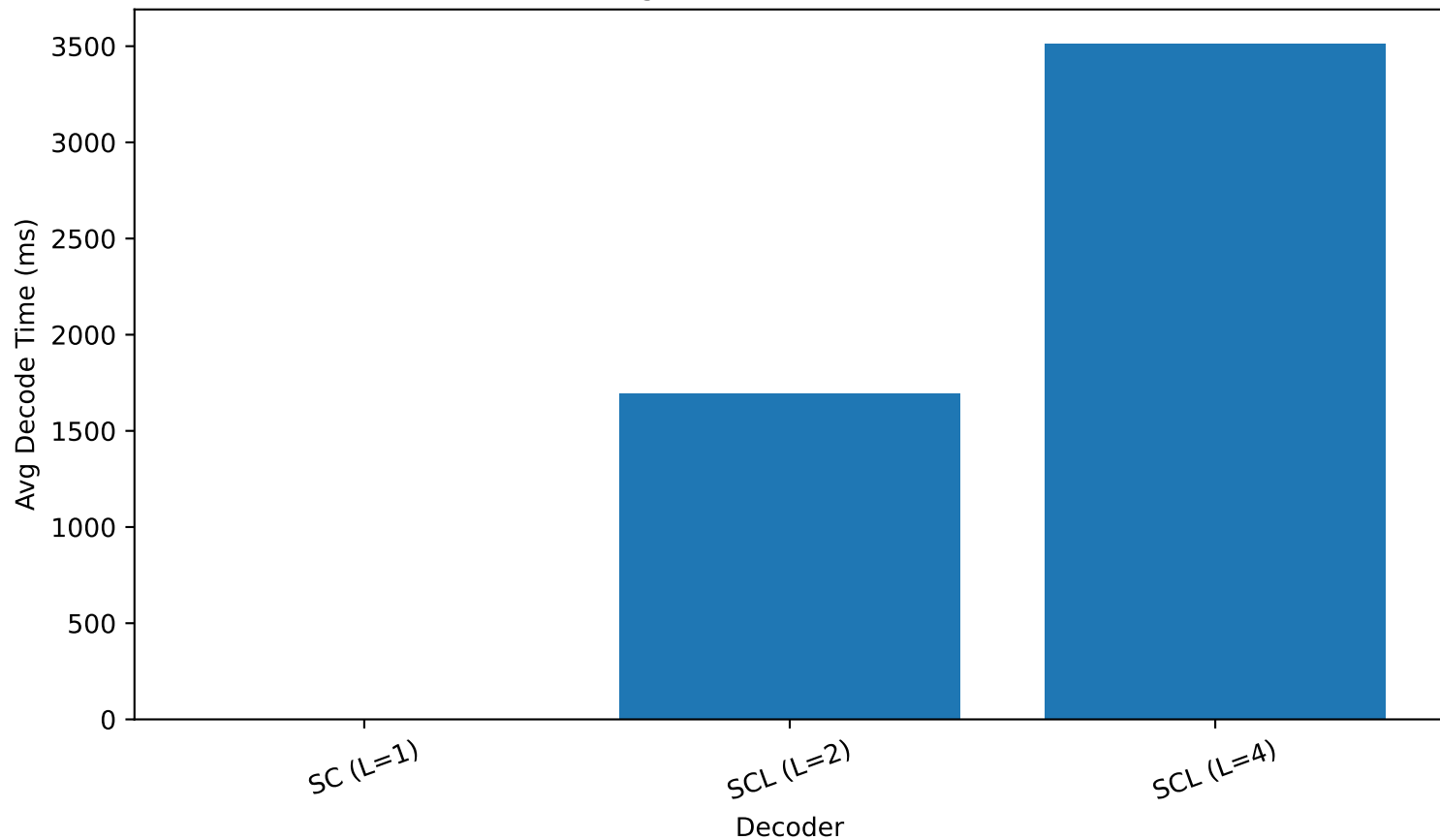
Decoding Time vs List Size (N=256)
