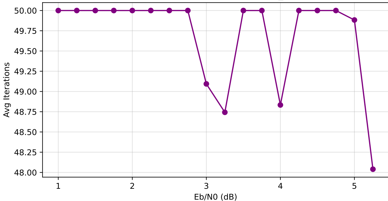
BP Average Iterations (N=256, max_iter=50)
