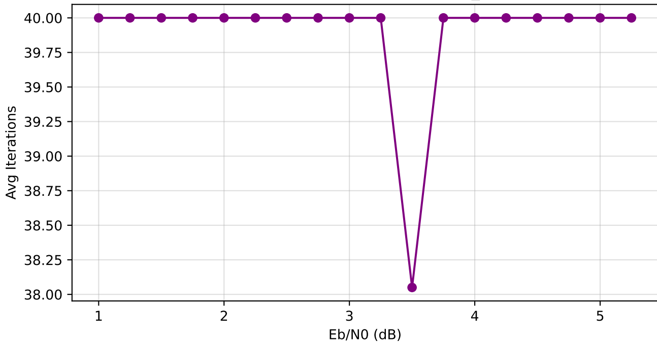
BP Average Iterations (N=512, max_iter=40)
