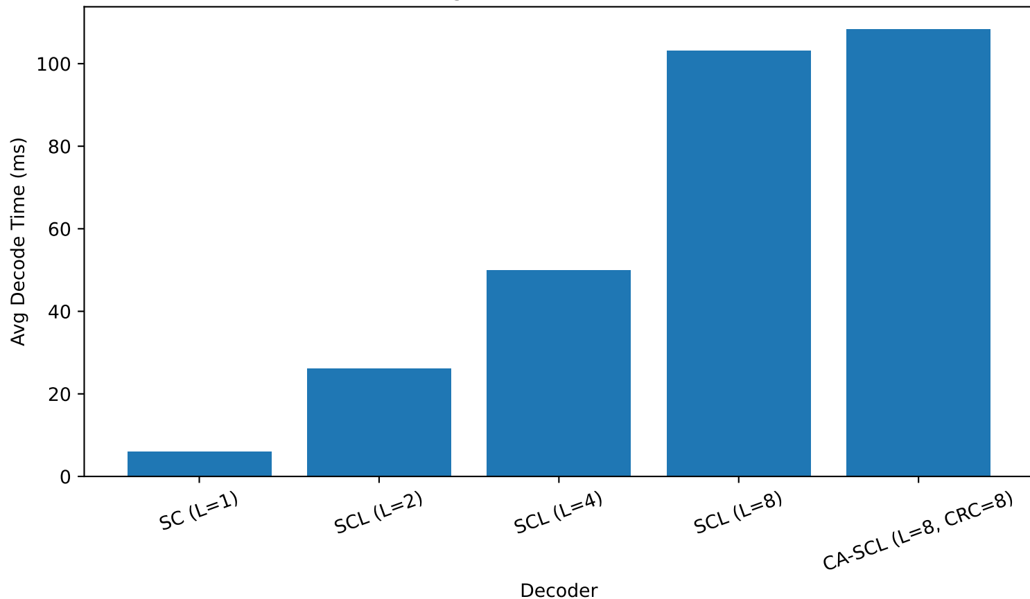
Decoding Time vs List Size (N=512)
