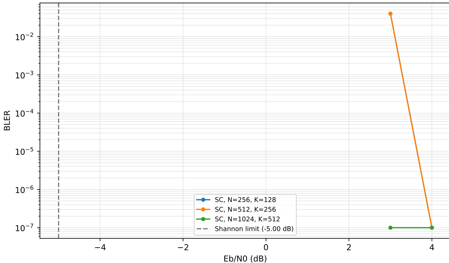
SC BLER (R=0.5)
