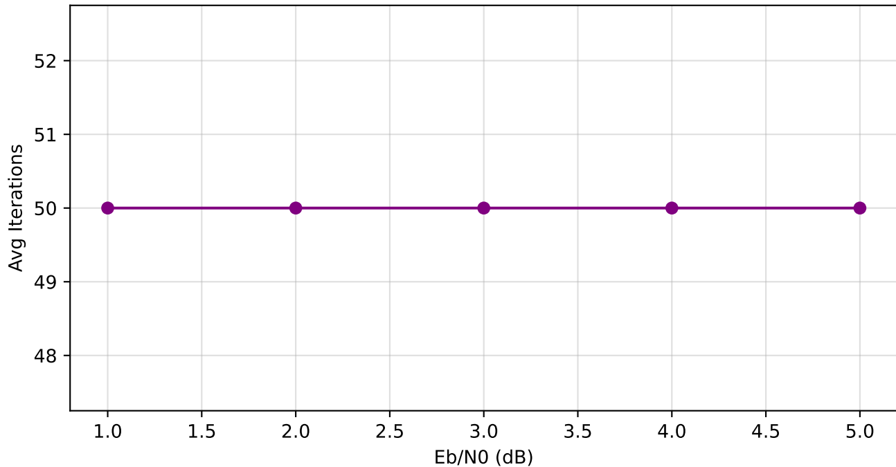
BP Average Iterations (N=32, max_iter=50)
