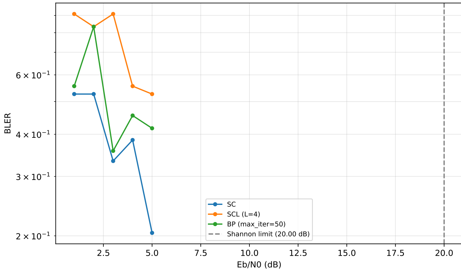
SC vs SCL vs BP (N=8, R=0.5)
