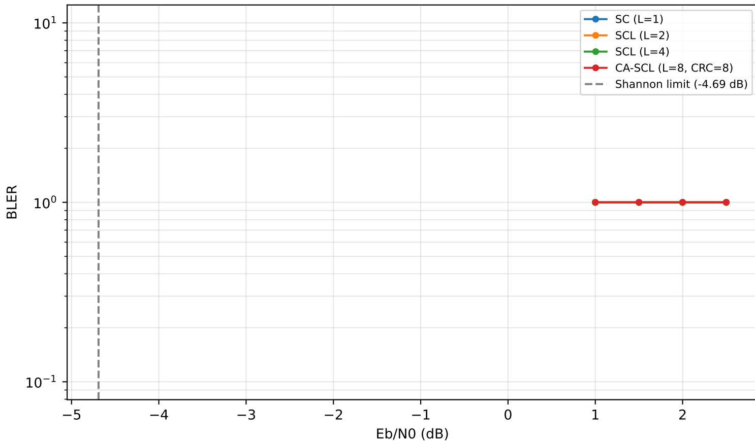
SCL vs SC BLER (N=256, R=0.5)
