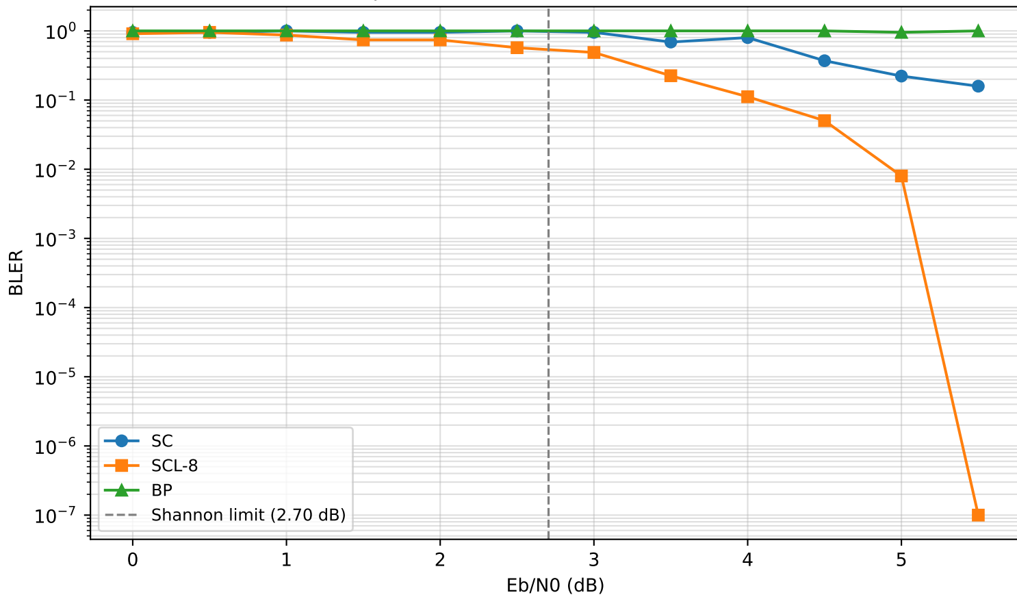
Exp1: SC vs SCL vs BP (N=128, K=64)
