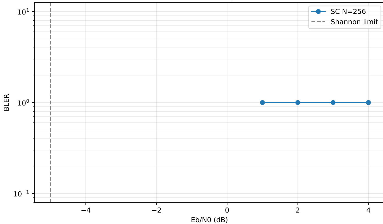
SC BLER (sample)
