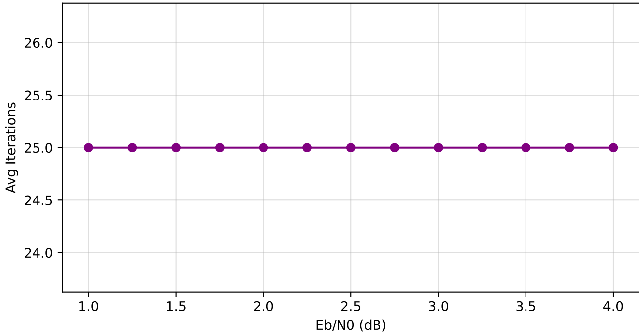
BP Average Iterations (N=512, max_iter=25)
