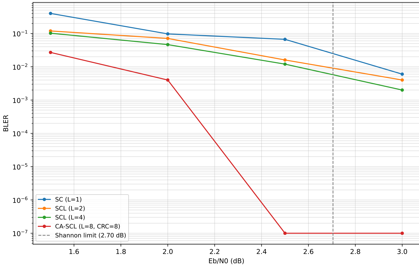
SCL vs SC BLER (N=256, R=0.5)
