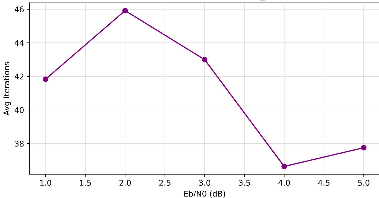
BP Average Iterations (N=8, max_iter=50)
