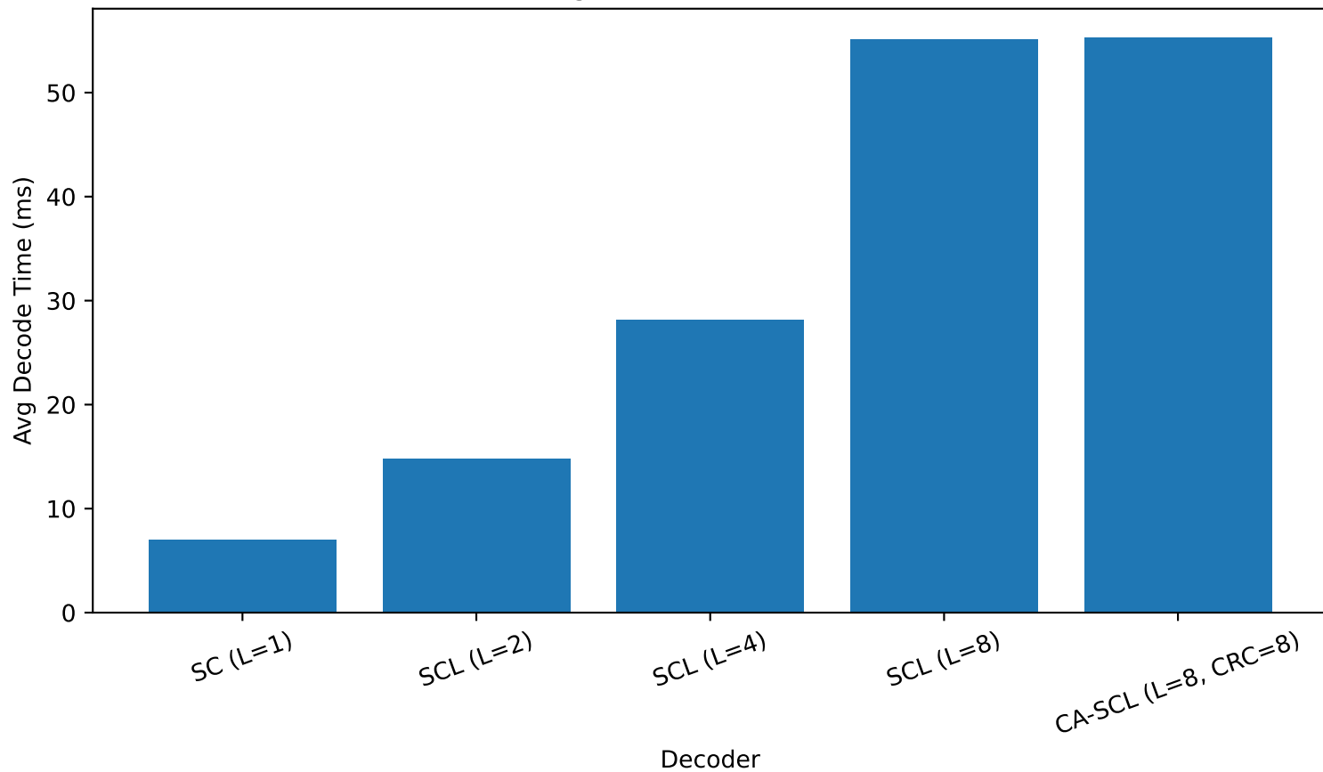
Decoding Time vs List Size (N=512)
