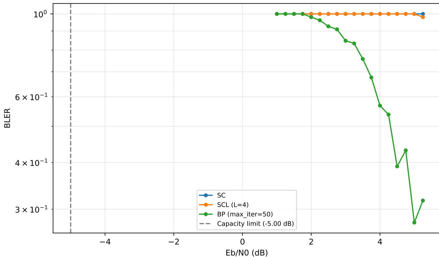
Decoder N=512
