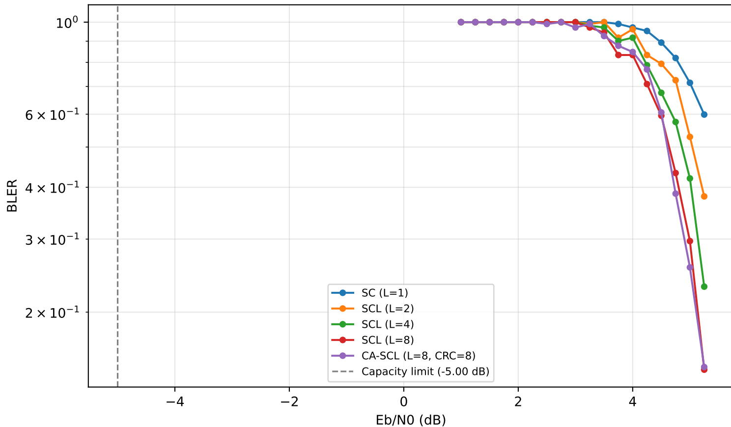
SCL vs SC BLER (N=512, R=0.5)
