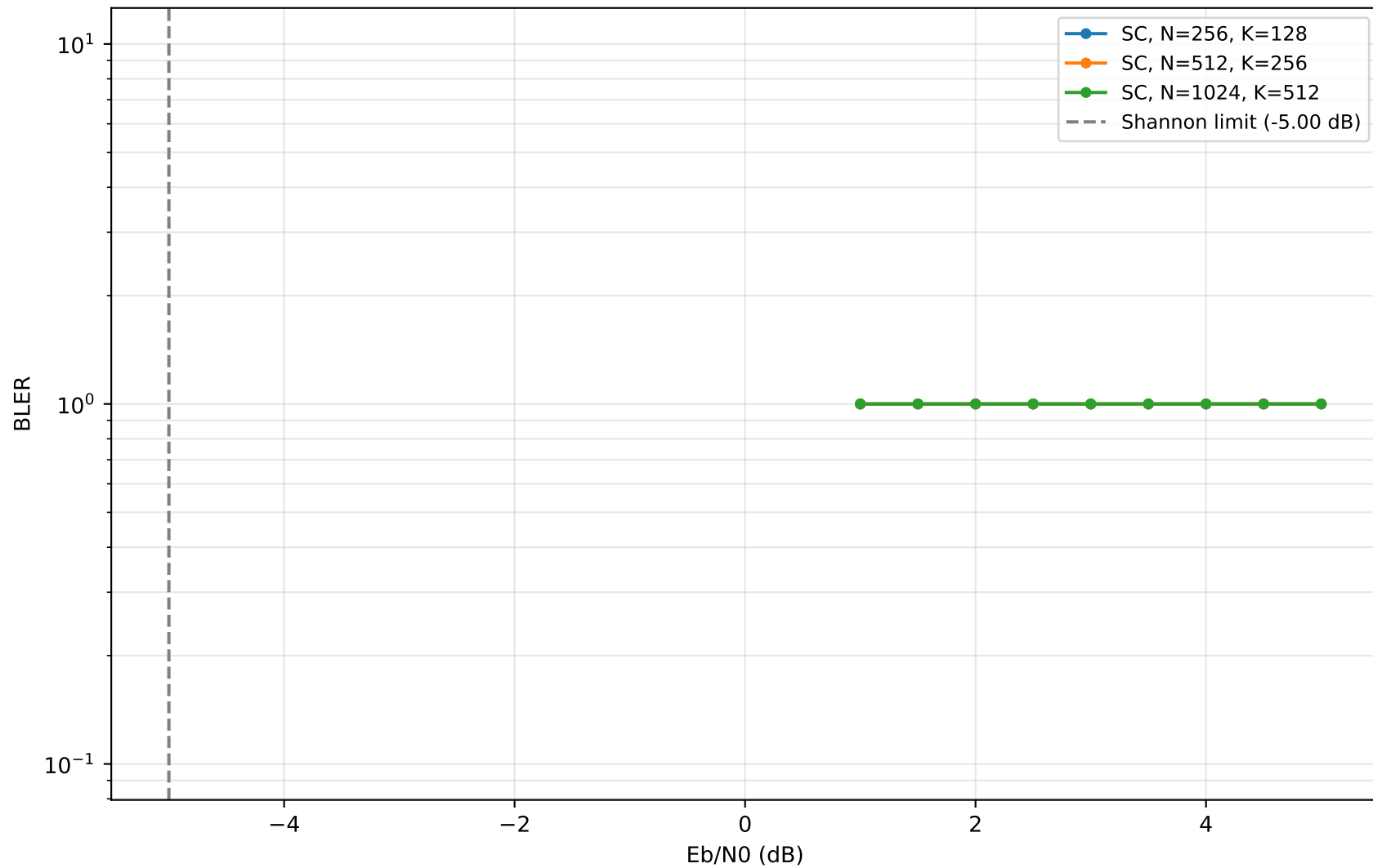
SC Decoder BLER (R=0.5)
