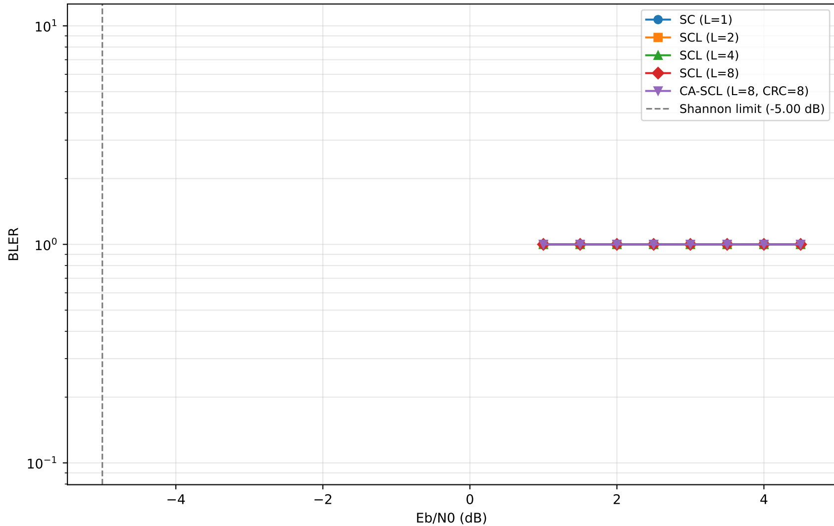
SCL BLER
