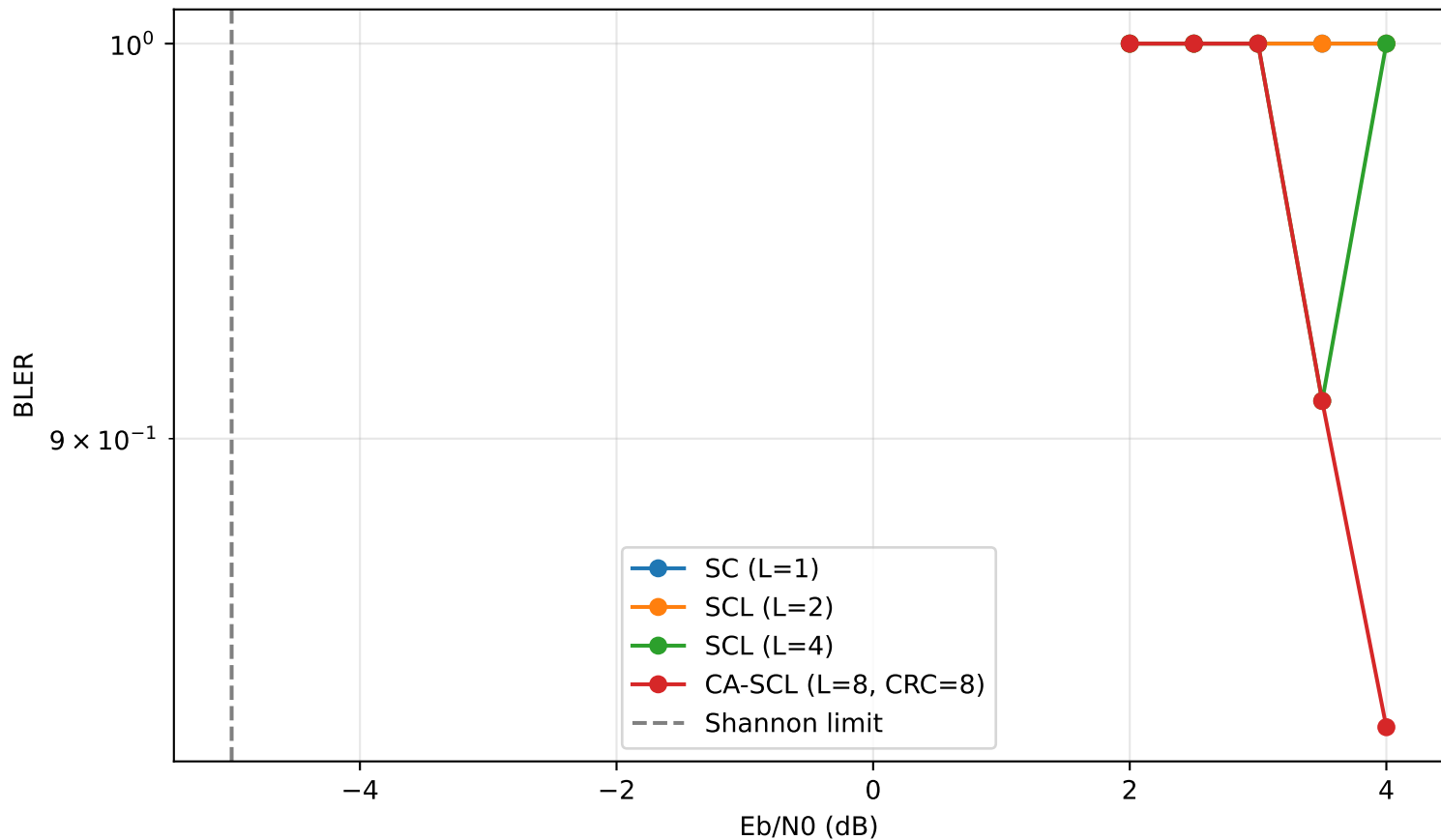
SCL vs SC BLER (N=128, R=0.5)
