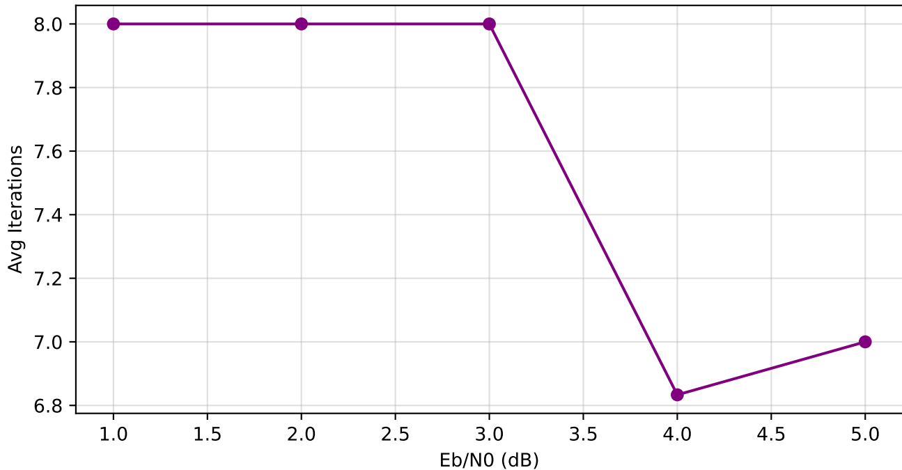
BP Average Iterations (N=256, max_iter=15)
