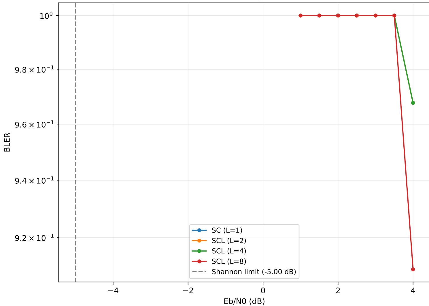
SCL BLER (quick)
