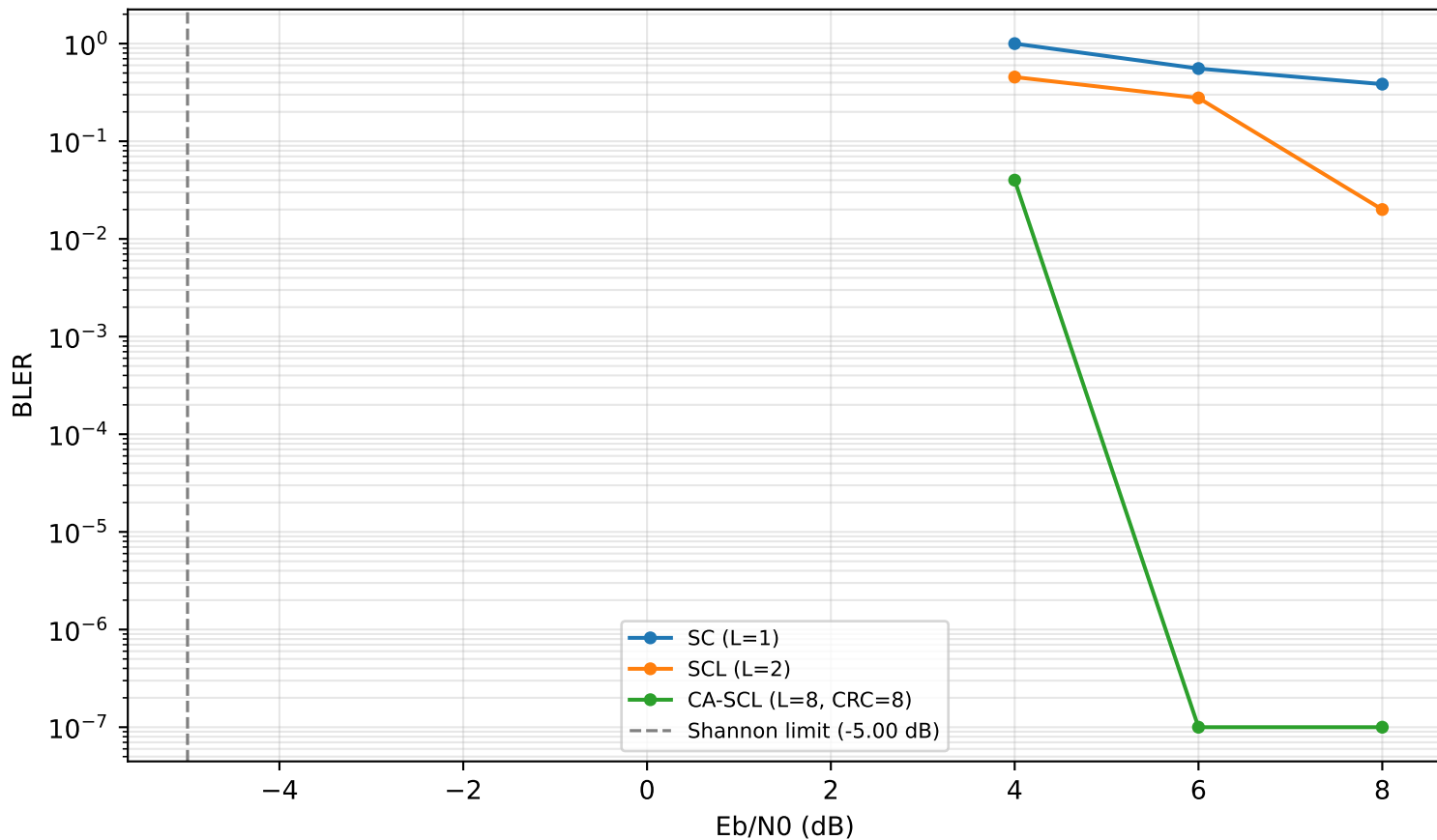
SCL vs SC BLER (N=64, R=0.5)
