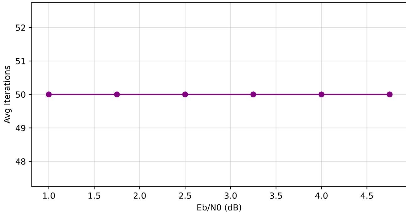
BP Average Iterations (N=128, max_iter=50)
