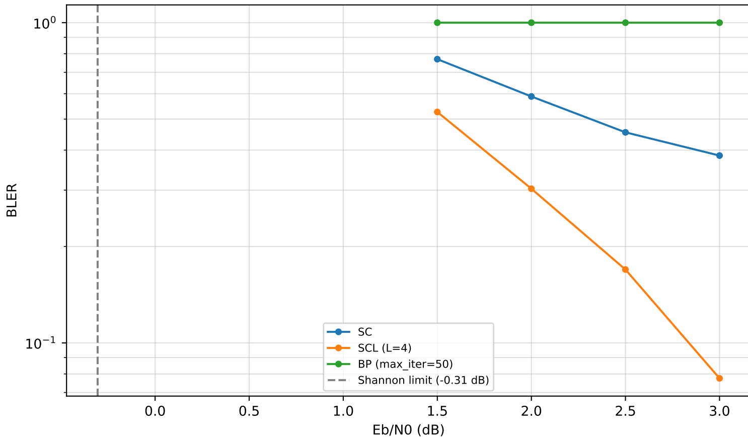
SC vs SCL vs BP (N=64)
